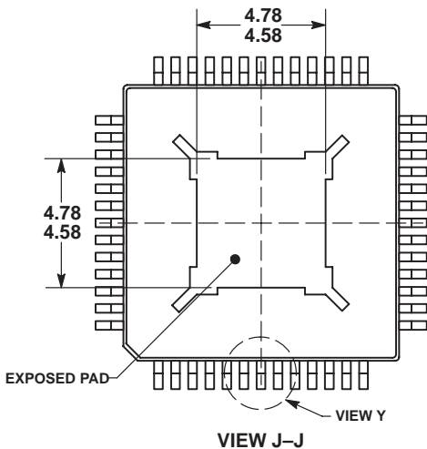
VIEW J-J
